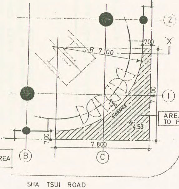
PART OF GROUND FLOOR PLAN
