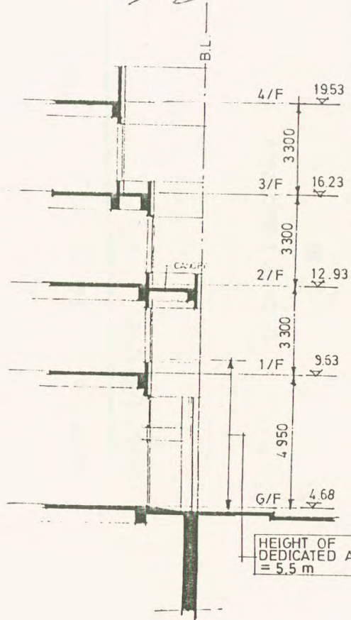
DIAGRAMMATIC SECTION
