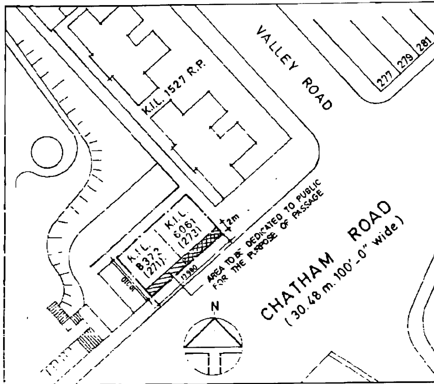
BLOCK PLAN
