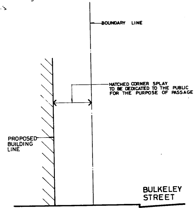
SECTION A SCALE 1:100
