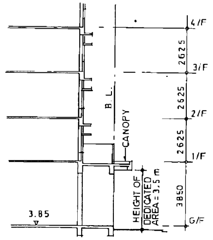
DIAGRAMMATIC SECTION SCALE 1:200
