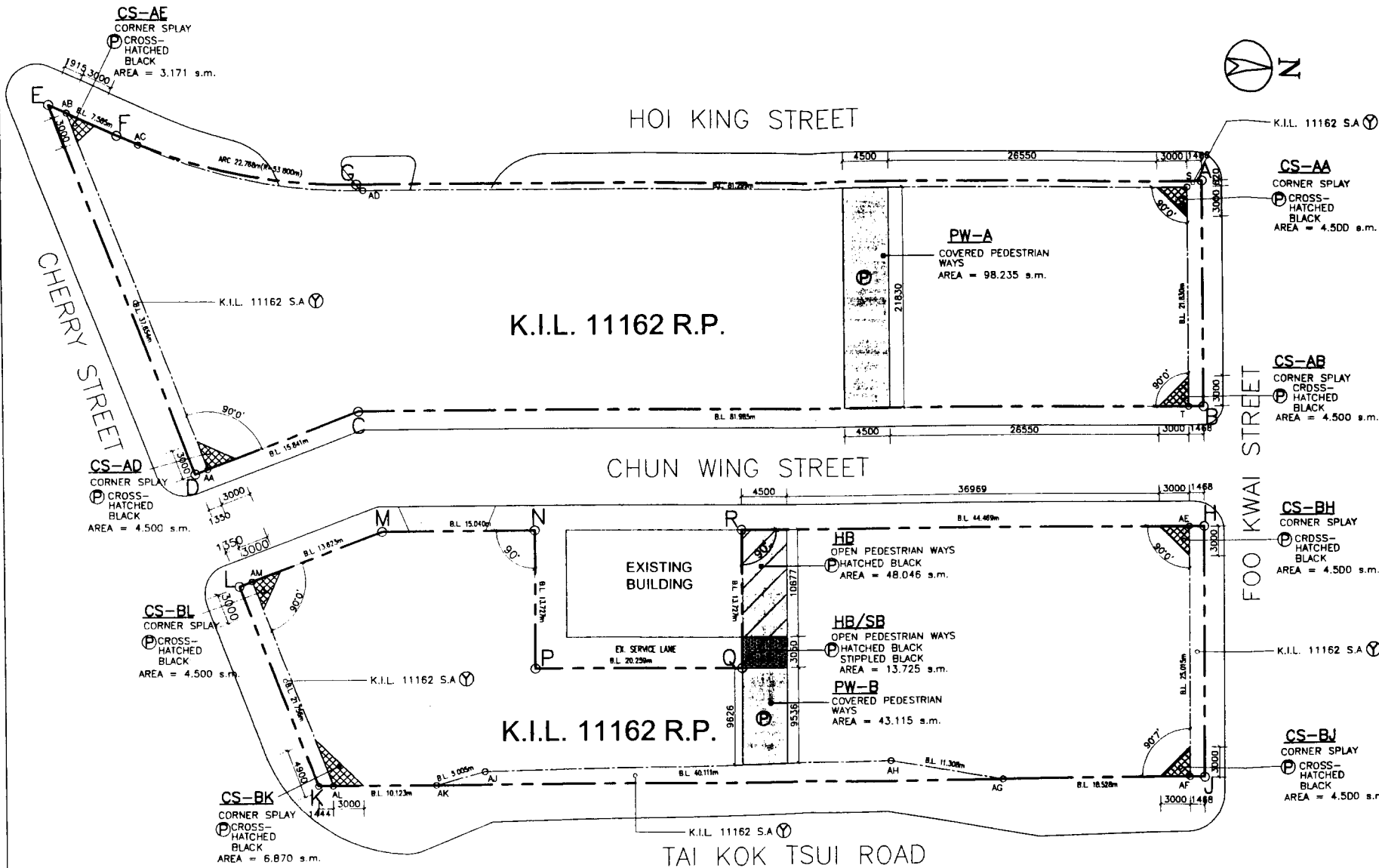
BLOCK PLAN 1: 4000
