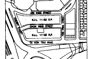
BLOCK PLAN 1: 4000
