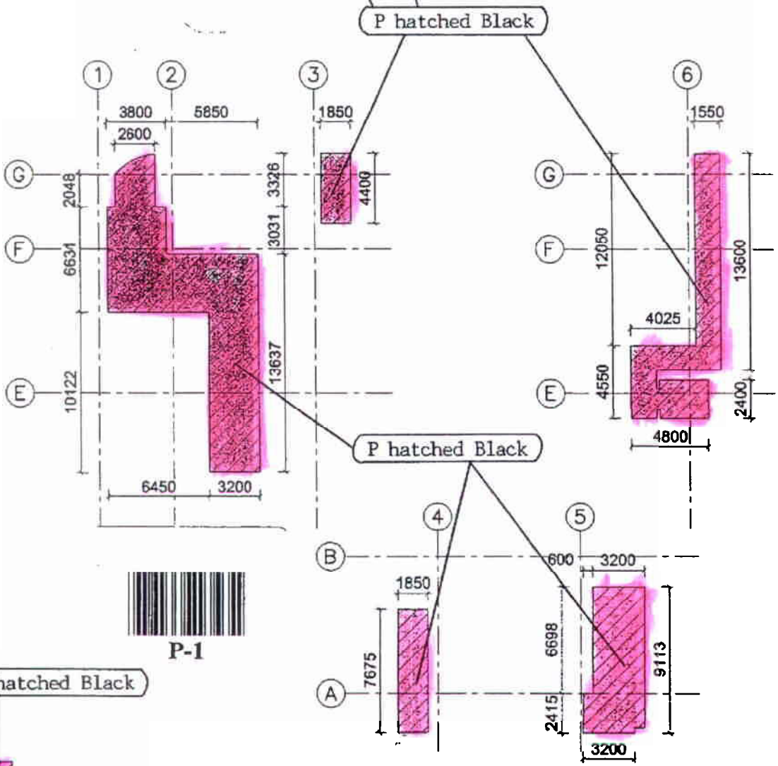
GROUND FLOOR DEDICATION AREA DIAGRAM
