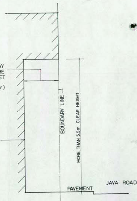
SECTION X' SCALE 1:100
