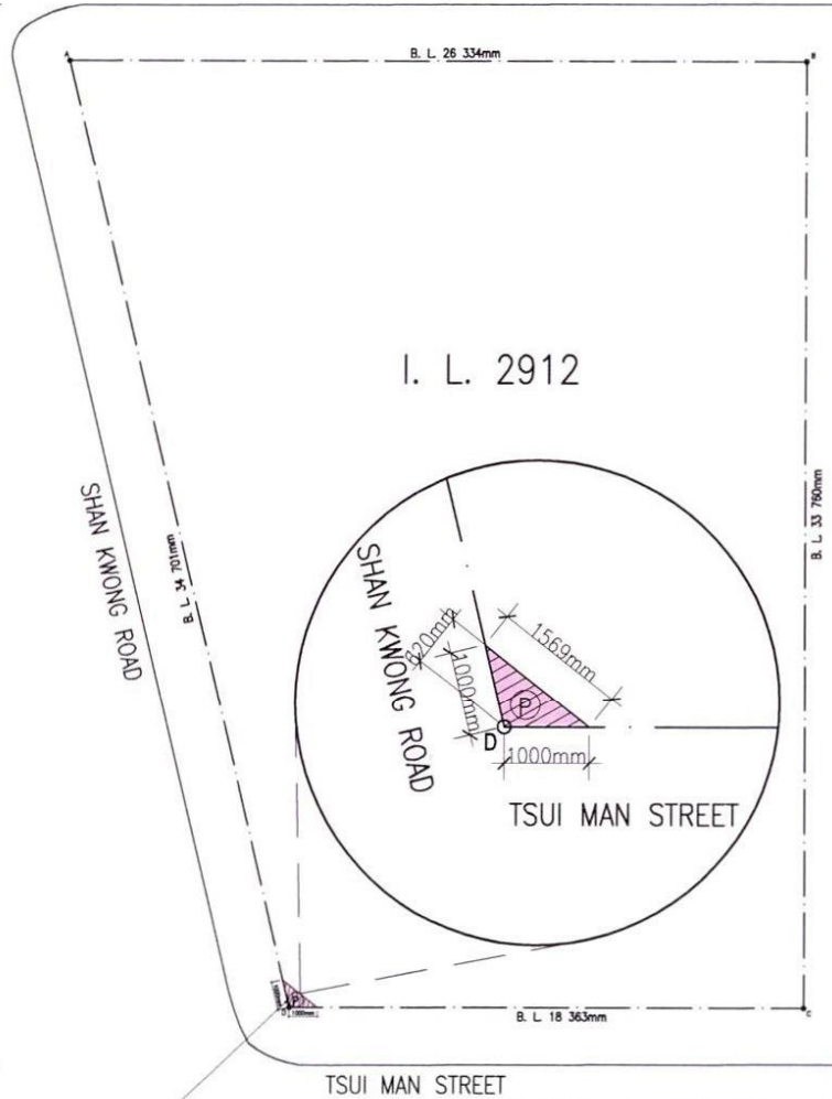
GROUND FLOOR PLAN (1:300)
