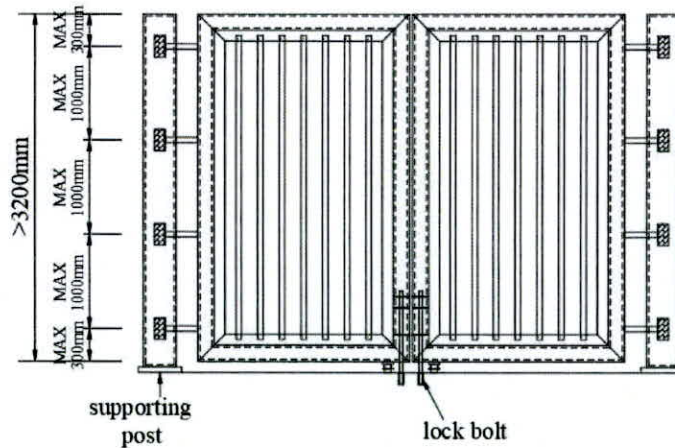
Swing-Type Metal Gate
