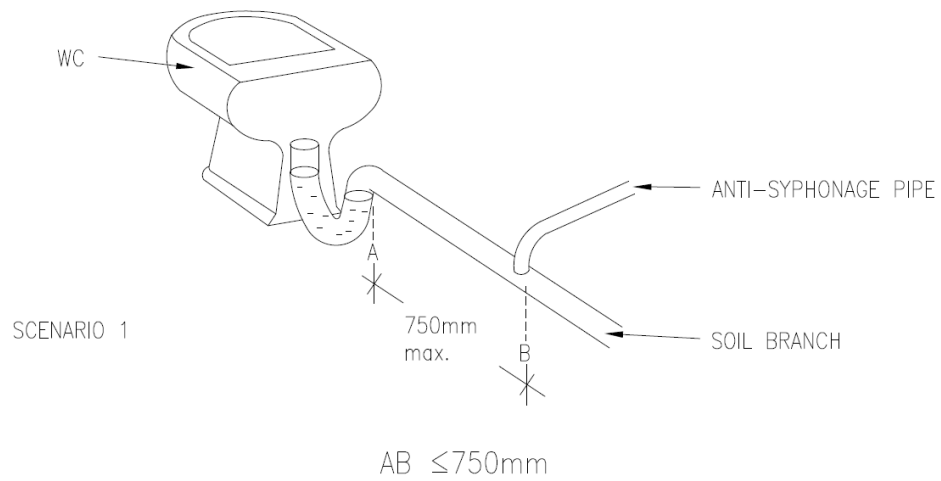
Figure 8: Maximum distance between trap outlet to anti-syphonage pipe
