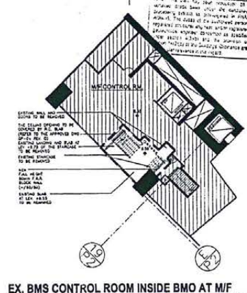
EX. BMS CONTROL ROOM INSIDE BMO AT M/F 1:200
