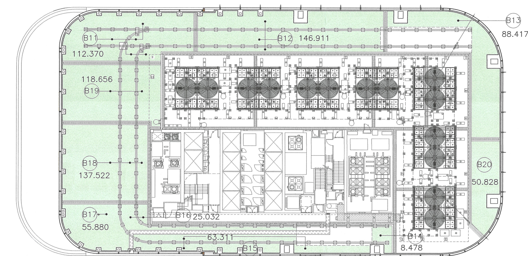
PHASE 2B BUILDING MAIN ROOF SCALE 1:300
