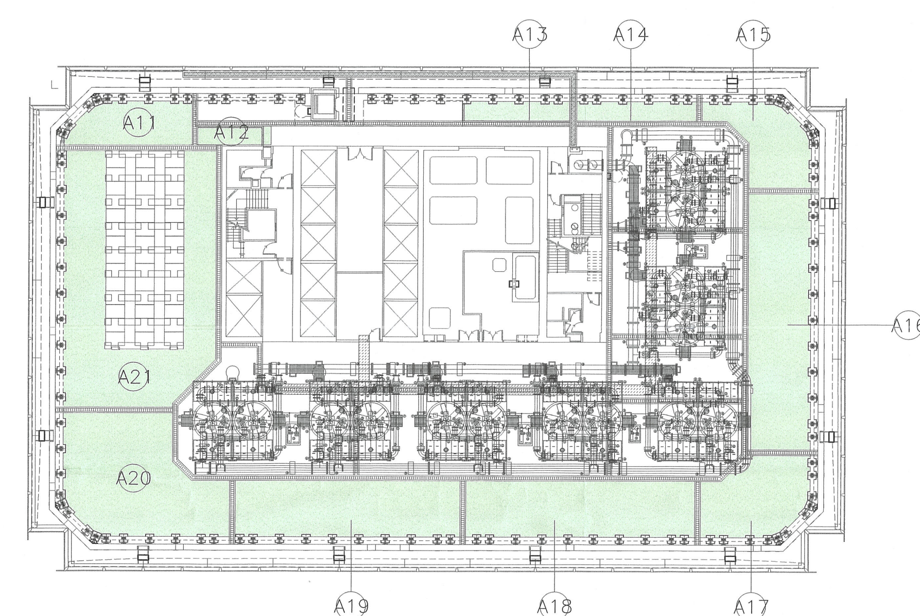
PHASE 2A BUILDING MAIN ROOF SCALE 1:300
