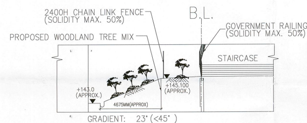
SECTION R-R 1:150
