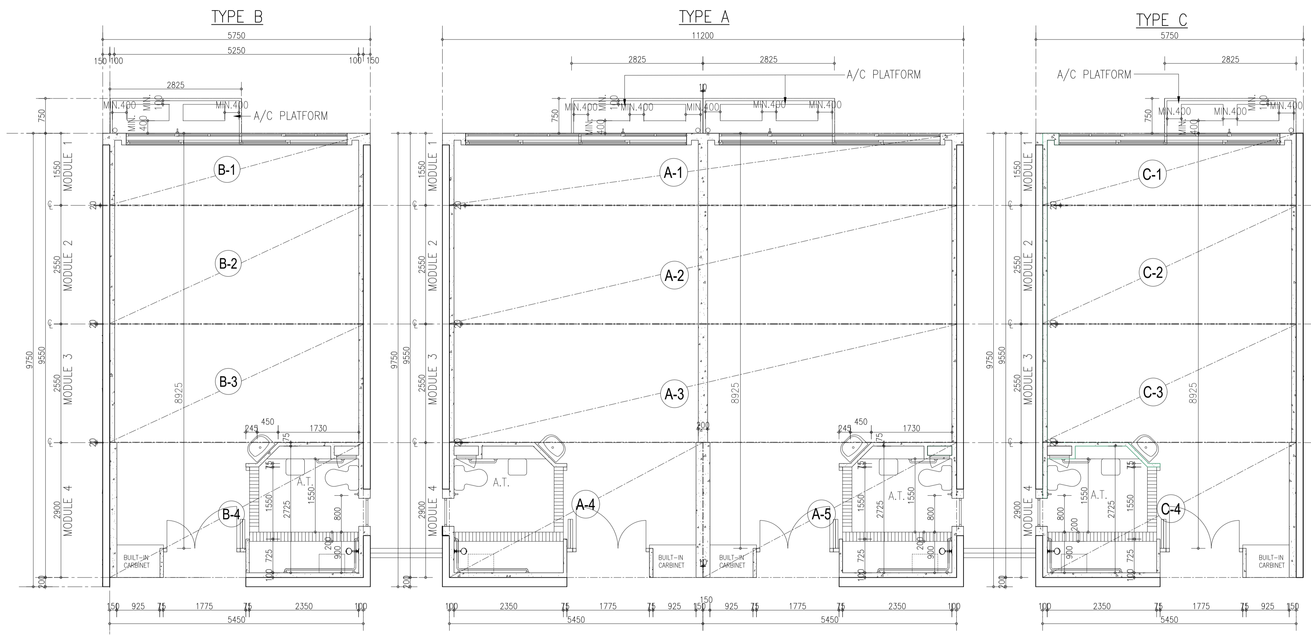
1 TYPE OF MIC BLOW UP PLAN 1:50
