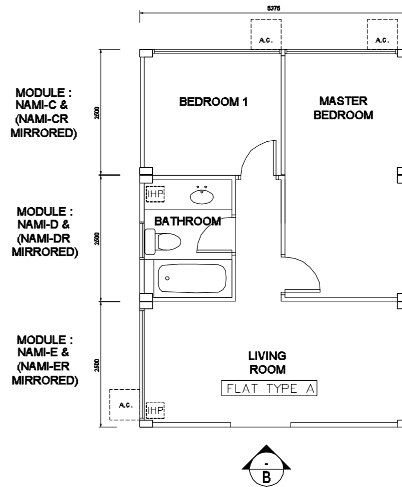
TYPICAL MODULE PLAN
