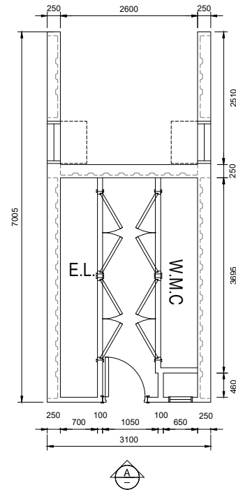
MiC MODULE EMR TYPE E
