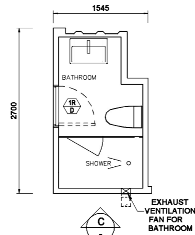
PLAN Module No. YLW-T03 Module No. (YLW-T03R) MIRRORED
