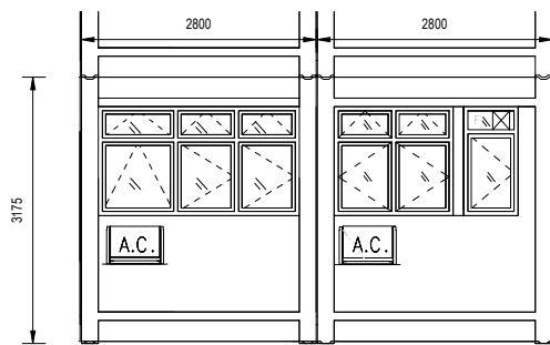
ELEVATION A (MODULE NO.: TYPE A & TYPE B)
