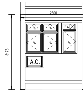
ELEVATION A (MODULE NO.: TYPE C)
