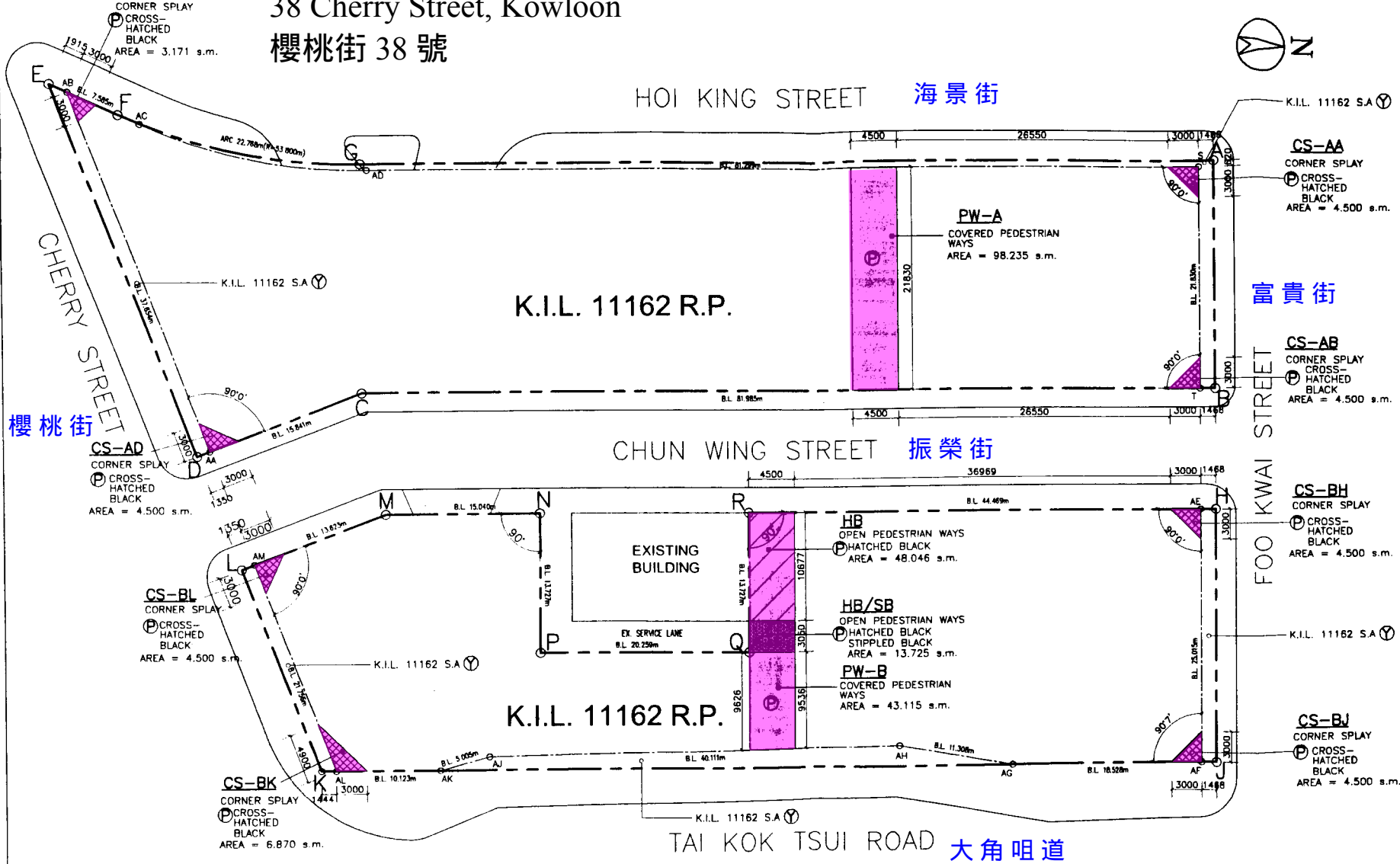
BLOCK PLAN 1: 4000
