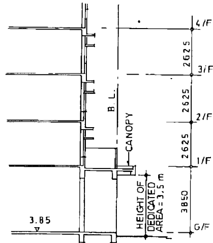
DIAGRAMMATIC SECTION SCALE 1:200
