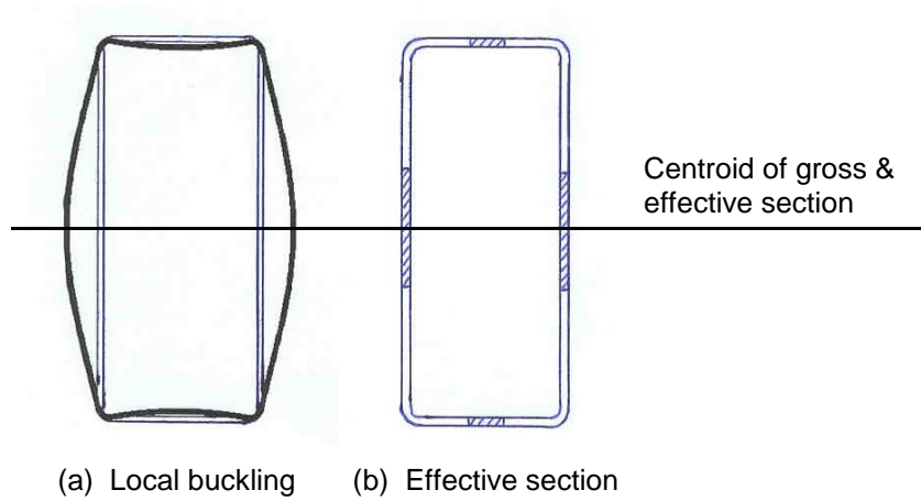
Figure 7.5 - Doubly symmetric slender cross-section subjected to compression
