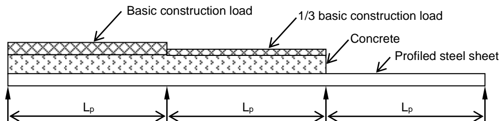
a) Arrangement for maximum negative moment
