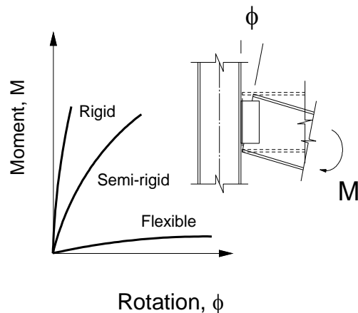
Figure 6.6 - Connection behaviour
