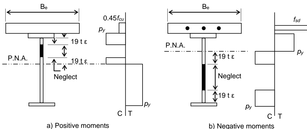
Figure 10.4 - Reduced section
