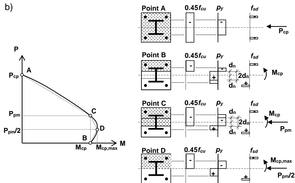
Figure 10.18 - Interaction curves and corresponding stress distributions
